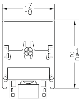
TRACK CROSS SECTION
