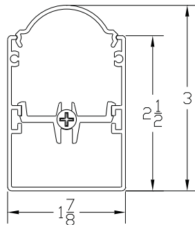
WIRE PASS CROSS SECTION
