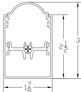
WIRE PASS CROSS SECTION
